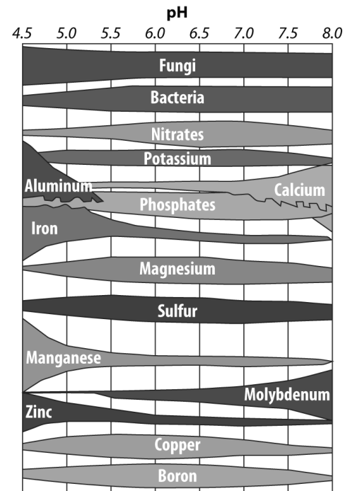
Figure 20.2. Effect of change in pH on the availability of plant nutrients.
