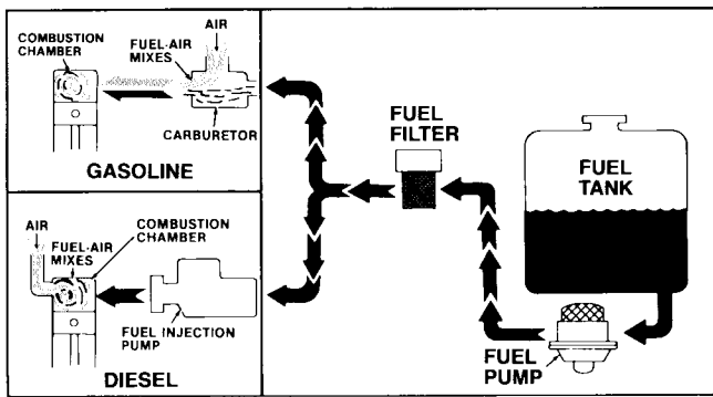
Figure 4-1 BASIC FUEL SYSTEM.
