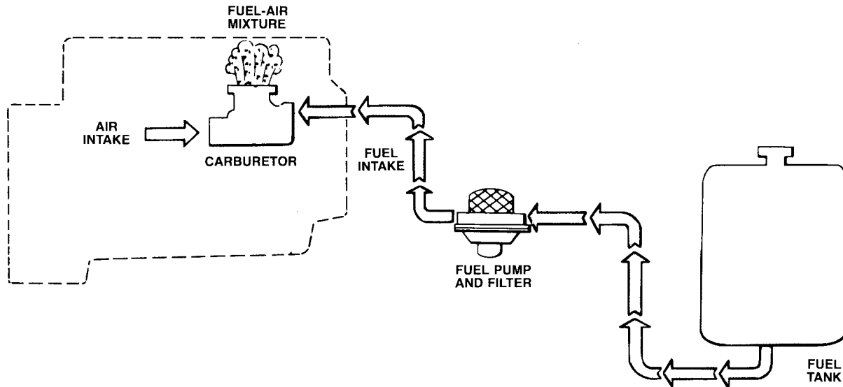
Figure 4-4 ARRANGEMENT OF COMPONENTS IN A GASOLINE FUEL SYSTEM — SPARK-IGNITION ENGINE.
