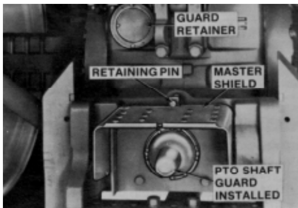
Figure 1-3 A SHIELD AND GUARD SHOULD COVER THE PTO SHAFT STUB.
