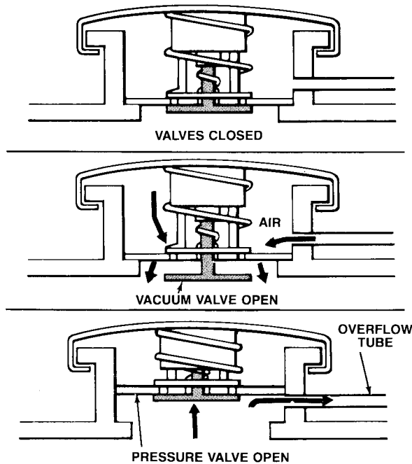
Figure 7-4 THE RADIATOR CAP MAINTAINS A PRE-SET PRESSURE WITHIN THE COOLING SYSTEM.
