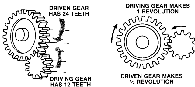
Figure 9-4 OUTPUT SPEED DEPENDS ON RELATIVE GEAR SIZE; SMALL GEAR ALWAYS TURNS FASTER.
