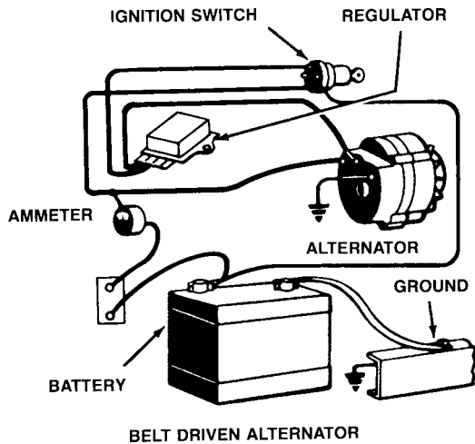
Figure 6-4 COMPONENTS OF AN ALTERNATING CURRENT (AC) CHARGING CIRCUIT.
