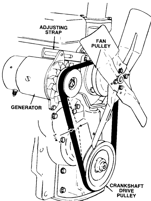
Figure 7-5 MAINTAIN PROPER TENSION ON THE FANBELT.
