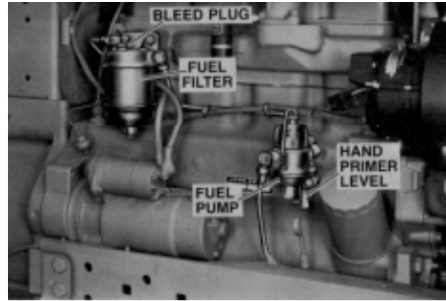
Figure 4-3 ONE TYPE OF ARRANGEMENT FOR BLEEDING A DIESEL FUEL SYSTEM ON A TRACTOR.
