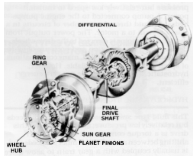
Figure 9-8 A TRACTOR FINAL DRIVE WITH PLANETARY GEAR ASSEMBLIES AT OUTER ENDS OF FINAL DRIVE SHAFTS.
