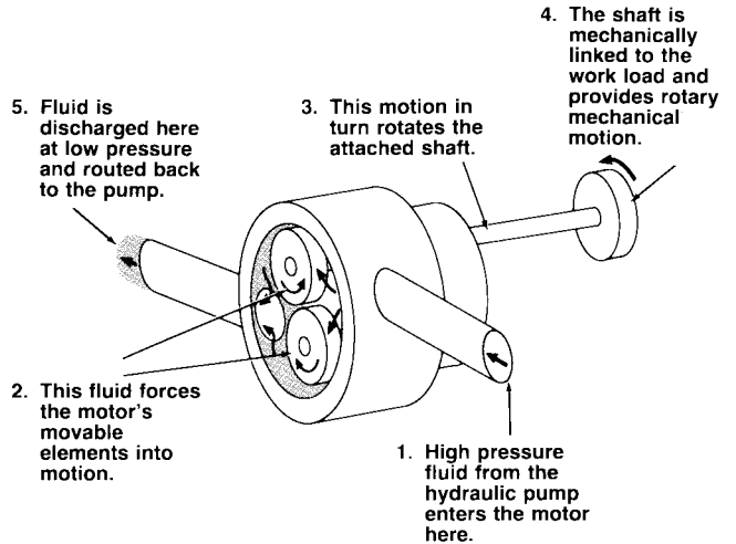
Figure 8-4 BASIC OPERATION OF A HYDRAULIC MOTOR.
