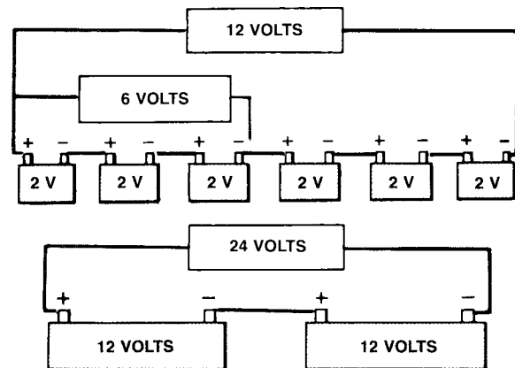
Figure 6-2 BATTERIES MAY BE CONNECTED TO PROVIDE ADDITIONAL ENERGY.
