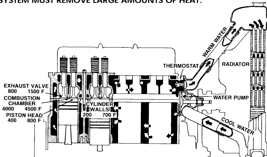
Figure 7-1 A COOLING SYSTEM MUST REMOVE LARGE AMOUNTS OF HEAT.
