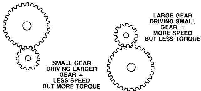
Figure 9-3 TORQUE VARIES WITH RELATIVE GEAR SIZE.
