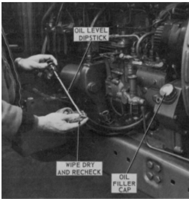
Figure 5-3 THE DIPSTICK IS USED TO CHECK THE ENGINE OIL LEVEL DAILY.
