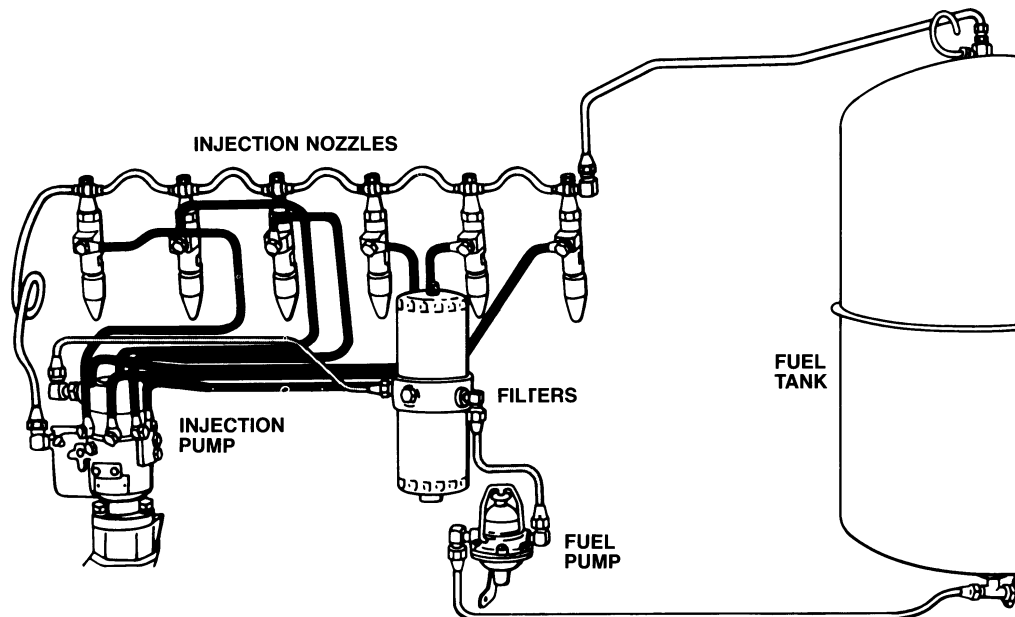
Figure 4-2 MAIN COMPONENTS OF A DIESEL FUEL SYSTEM (DISTRIBUTOR TYPE SHOWN).
