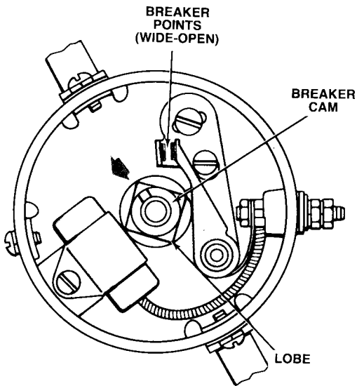
Figure 6-6 DISTRIBUTOR BREAKER POINTS OPENED BY THE BREAKER CAM. (HOW MANY CYLINDERS DOES THIS ENGINE HAVE?)
