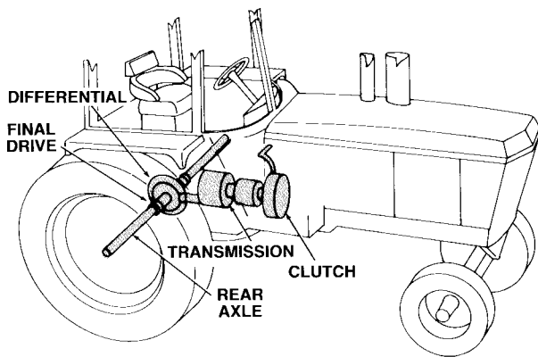
Figure 9-1 LOCATION OF COMPONENTS OF THE POWER TRAIN IN A TRACTOR.
