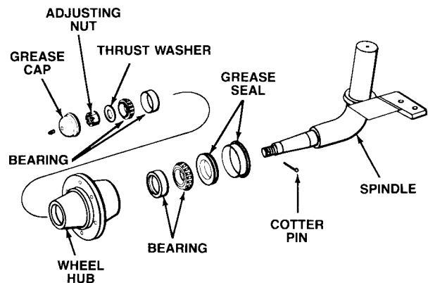
Figure 5-5 BEARINGS ON A SPINDLE WHEEL ASSEMBLY.
