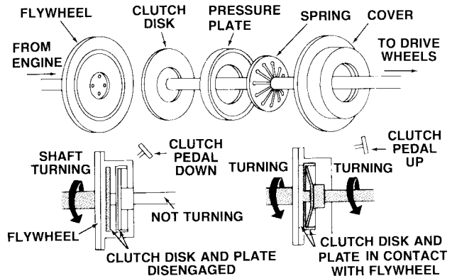
Figure 9-2 PARTS OF A SIMPLE DISK CLUTCH.
