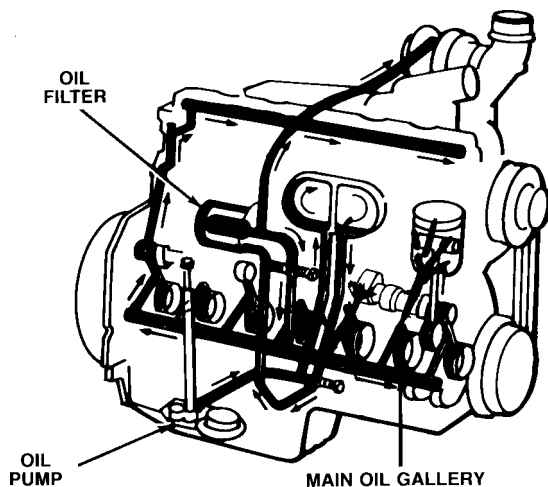
Figure 5-1 A FULL-FORCE FEED LUBRICATION SYSTEM FOR A TRACTOR ENGINE.
