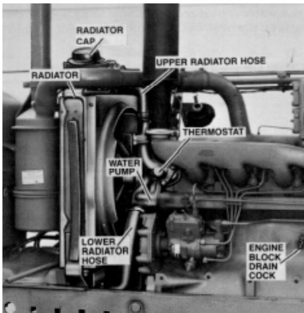
Figure 7-2 LIQUID COOLING SYSTEM ON A MODERN ENGINE.
