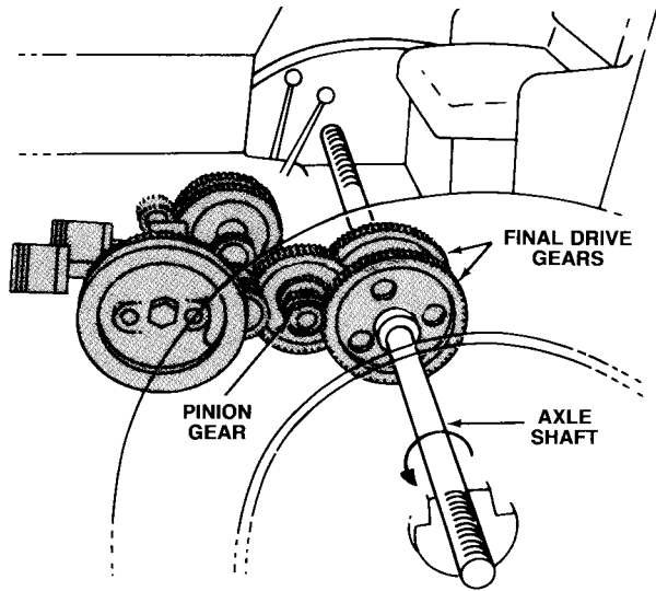
Figure 9-7 A PINION GEAR ASSEMBLY FOR SPEED REDUCTION LOCATED IN THE DIFFERENTIAL.
