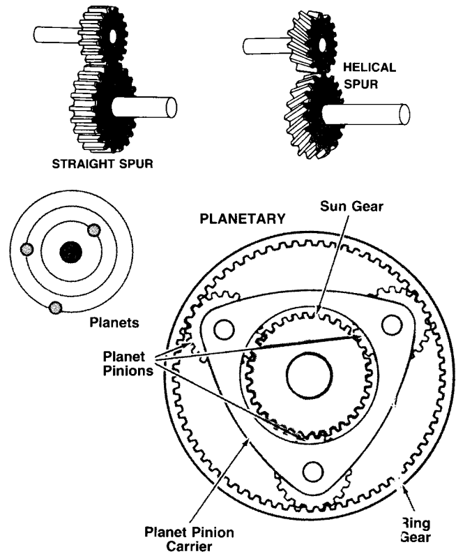
Figure 9-5 THREE TYPES OF GEARS COMMONLY FOUND IN TRACTOR TRANSMISSIONS.
