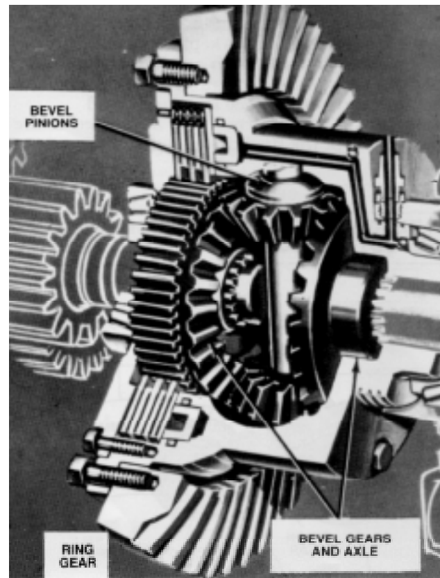
Figure 9-6 THE TRACTOR DIFFERENTIAL.
