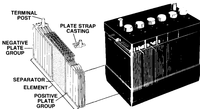
Figure 6-1 INTERNAL CONSTRUCTION OF A WET-CELL STORAGE BATTERY.
