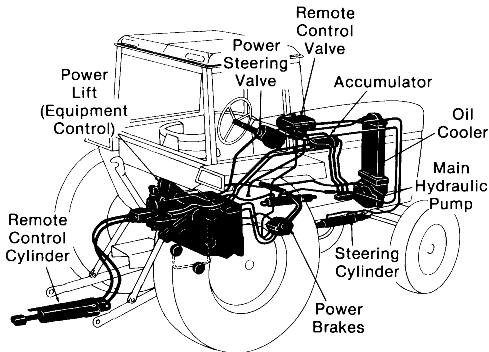
Figure 8-1 A MODERN TRACTOR WITH A COMPLETE HYDRAULIC SYSTEM.
