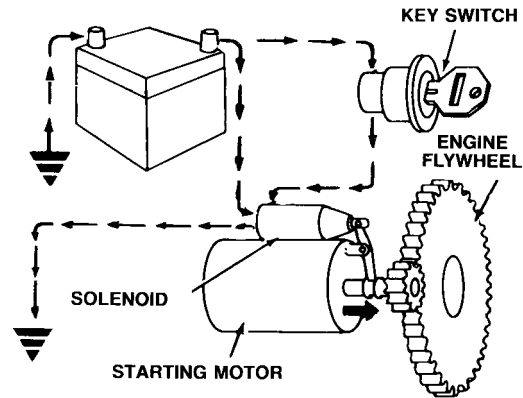
Figure 6-3 COMPONENTS OF AN ENGINE STARTING SYSTEM.
