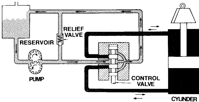
Figure 8-3 A SIMPLE HYDRAULIC SYSTEM.
