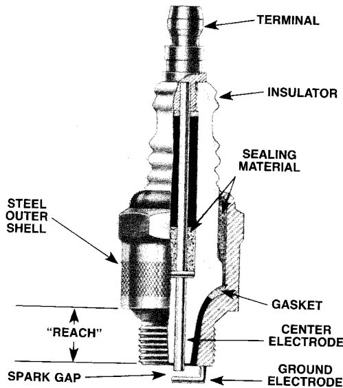
Figure 6-7 CUTAWAY VIEW OF A SPARK PLUG.
