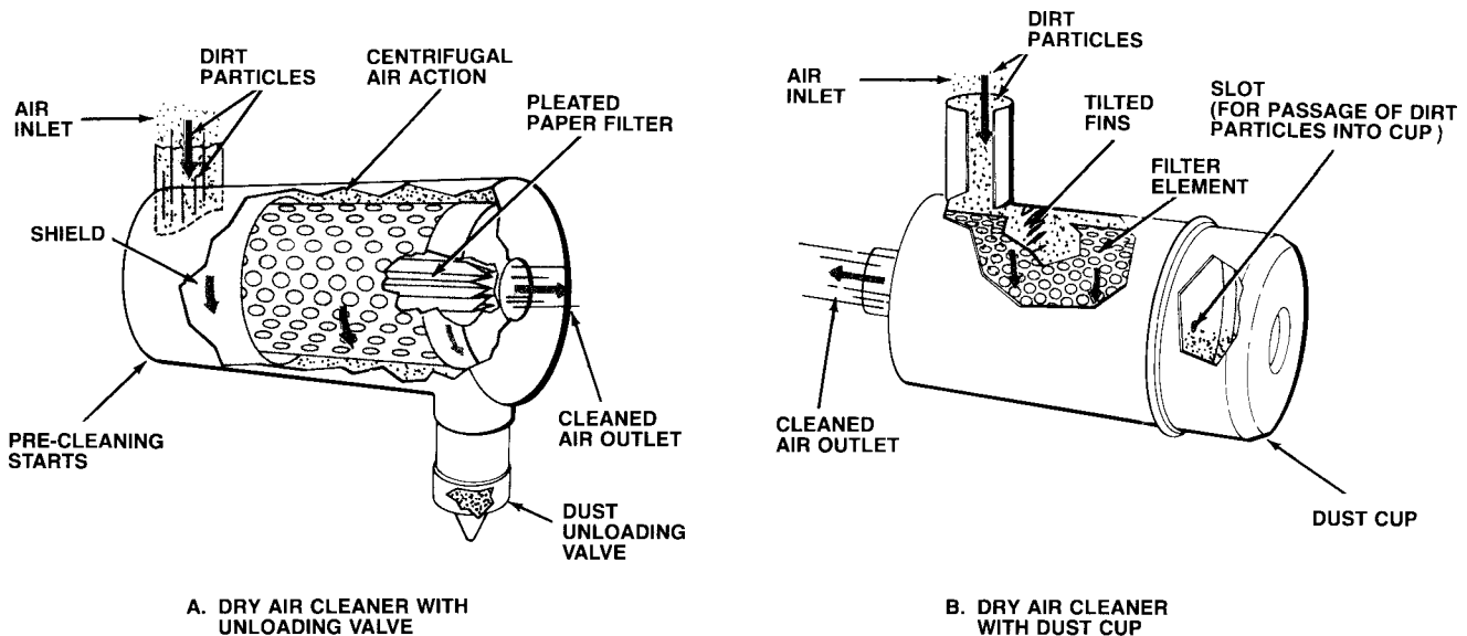
Figure 4-7 TWO METHODS OF REMOVING DUST WITH PRE-CLEANERS AND DRY-ELEMENT AIR CLEANERS.
