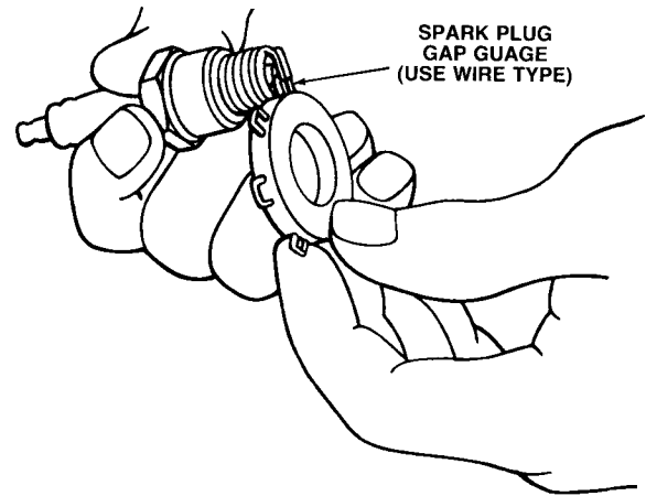
Figure 6-8 CHECKING THE SPARK PLUG GAP WITH A WIRE GAUGE.
