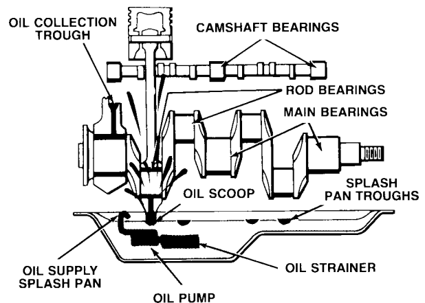
Figure 5-2 A CIRCULATING SPLASH LUBRICATING SYSTEM.
