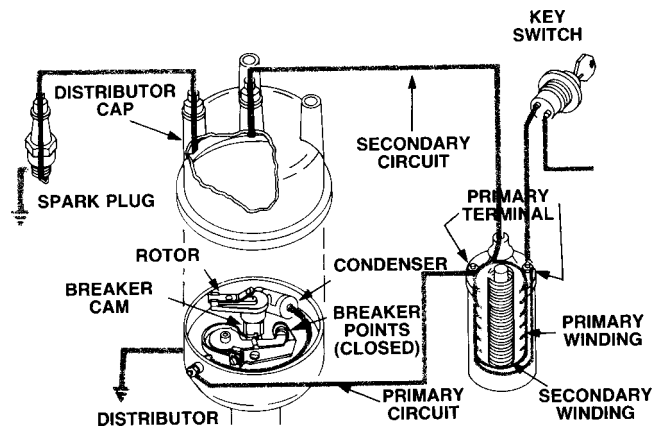
Figure 6-5 COMPONENTS OF PRIMARY AND SECONDARY SPARK-IGNITION CIRCUITS.
