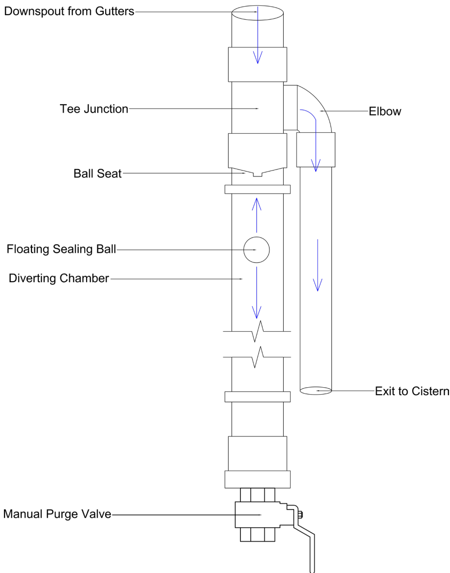
Figure 4. A flush diverter is a chamber with a floating ball valve at the top that fills prior to the main storage tank when the system collects water during a storm. The “first flush” is then purged to prevent contaminants from the initial roof wash from entering the main storage tank.
