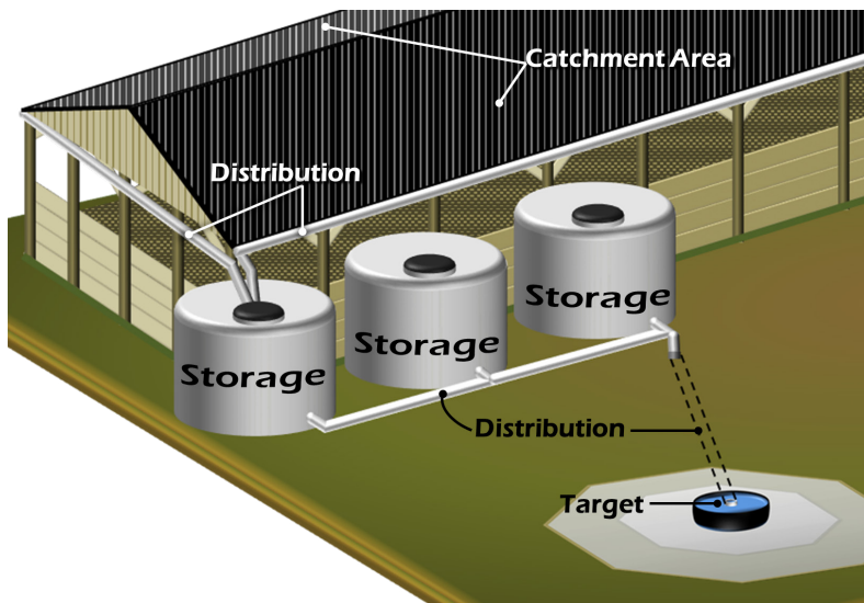
Figure 2. A basic design consists of a catchment area, distribution, storage, and a target. Figure by Donnie Stamper
